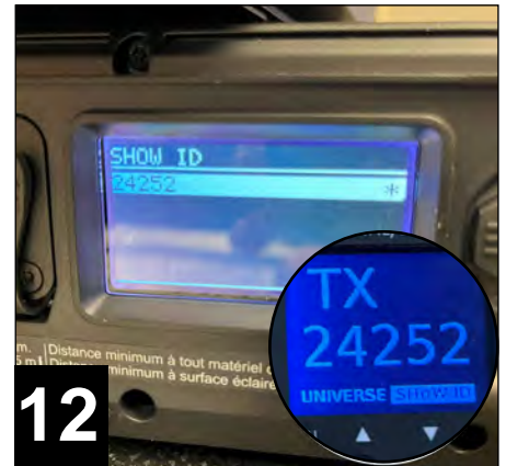
12. Confirm the SHoW ID and SHoW Key match the Multiverse Node, or other wireless DMX transceiver, settings.
